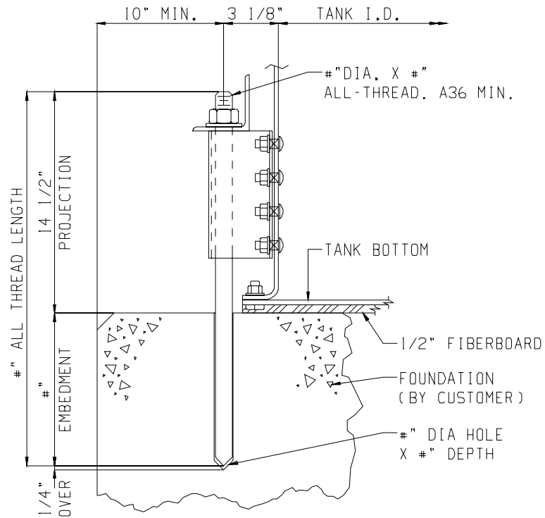
EPOXY ANCHOR BOLT DETAIL
